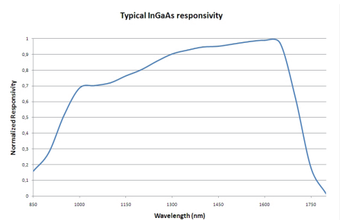
Typical Camera Spectral Sensitivity
